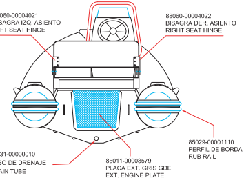
AFT VIEW
