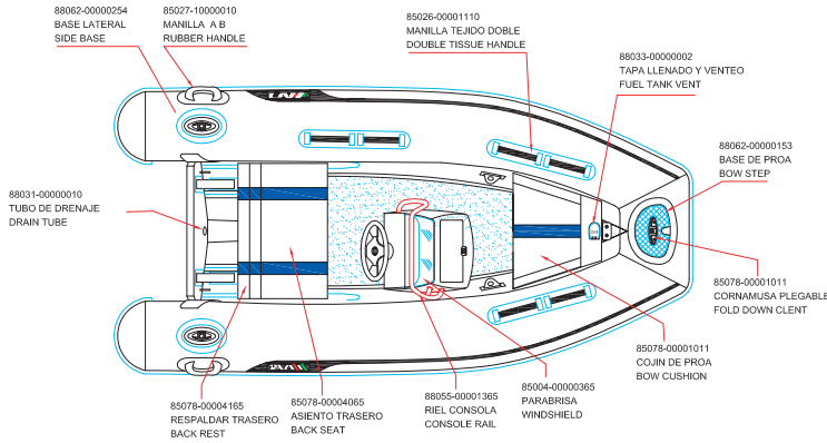
PLANT VIEW
