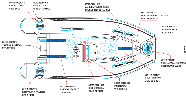
PLANT VIEW
