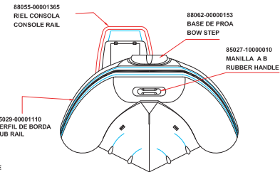
FORE VIEW
