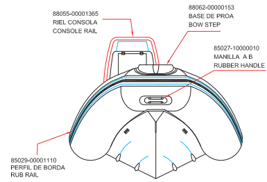
FORE VIEW
