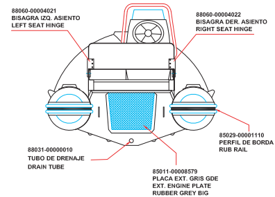
AFT VIEW
